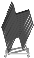
t35 and t35k Seat upholstered max 10 pcs Without upholstery max 15 pcs Size: 62 x 96 x 158 cm Weight: 20 + 60 kg
